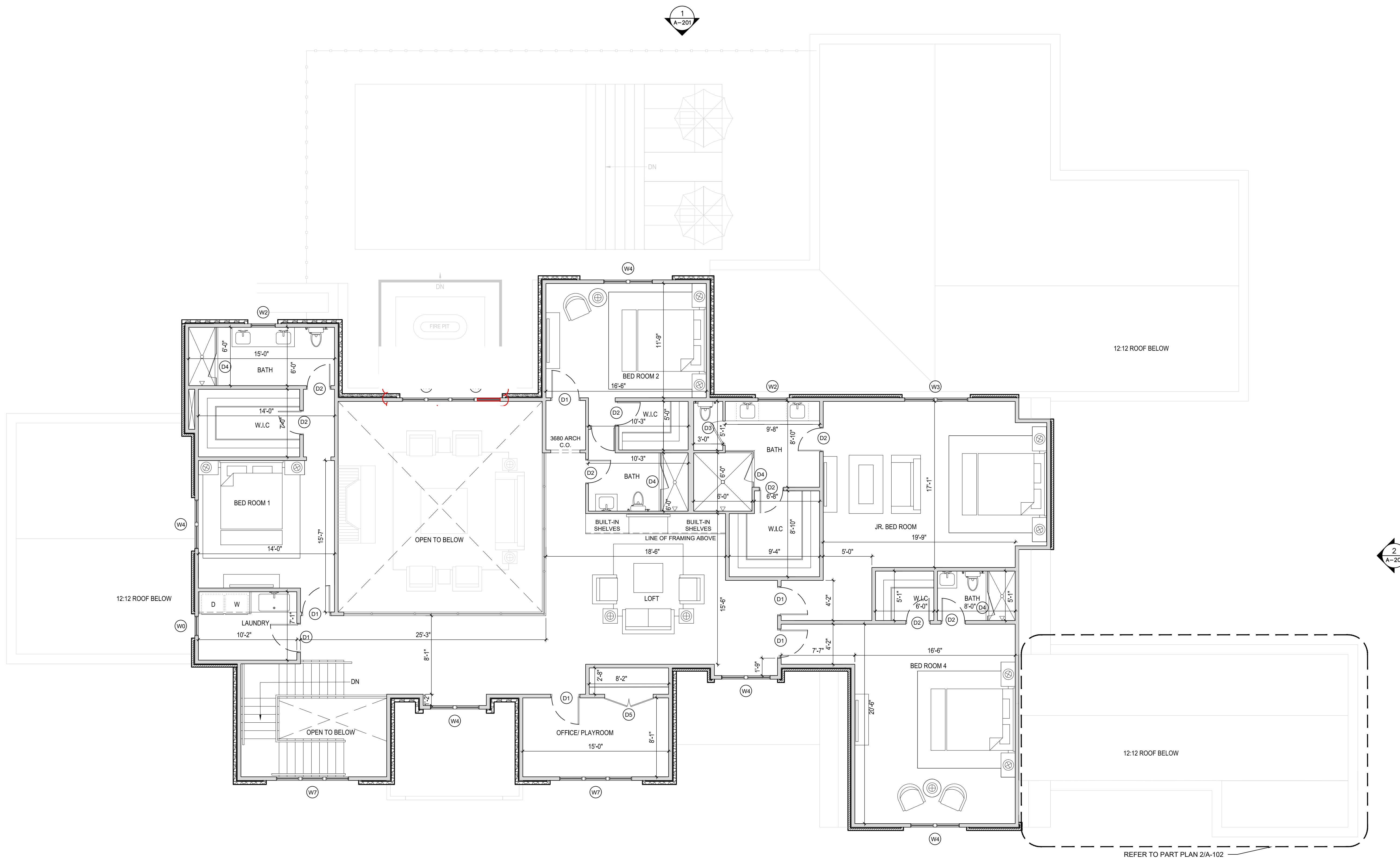
1 SECOND LEVEL FLOOR PLAN 3/16"=1'-0"
